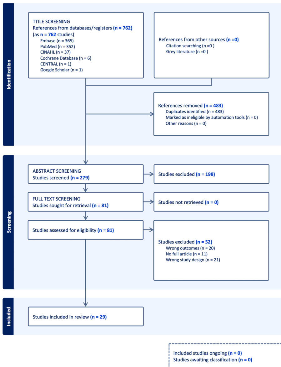
FIGURE 1: PRISMA chart
