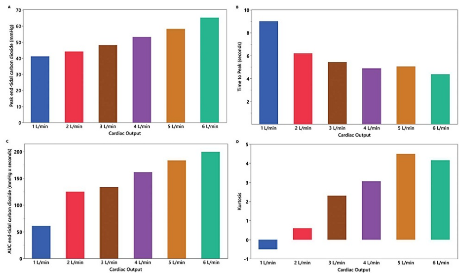
FIGURE 3: Graphical visualizations
