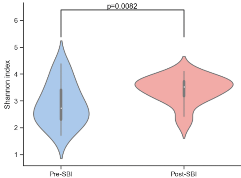
FIGURE 4: Alpha diversity at the genus level for pre-SBI and post-SBI using the Shannon diversity index.
