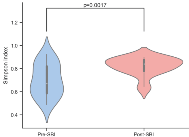
FIGURE 5: Alpha diversity at the genus level for pre-SBI and post-SBI using the Gini-Simpson diversity index.
