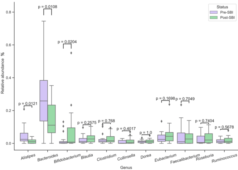
FIGURE 2: Relative abundances (%) of bacteria before and after SBI treatment at the genus level.
