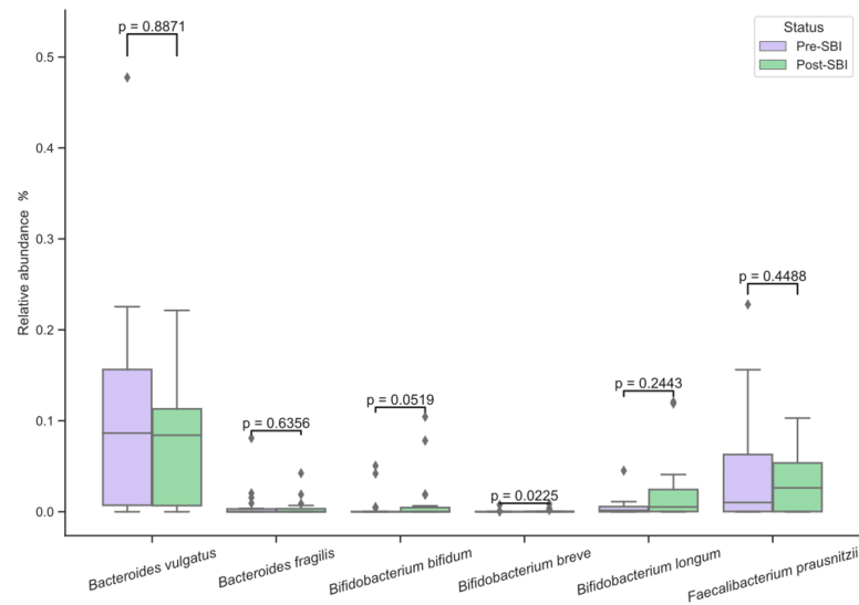
FIGURE 3: Relative abundances (%) of bacteria before and after SBI treatment at the species level.
