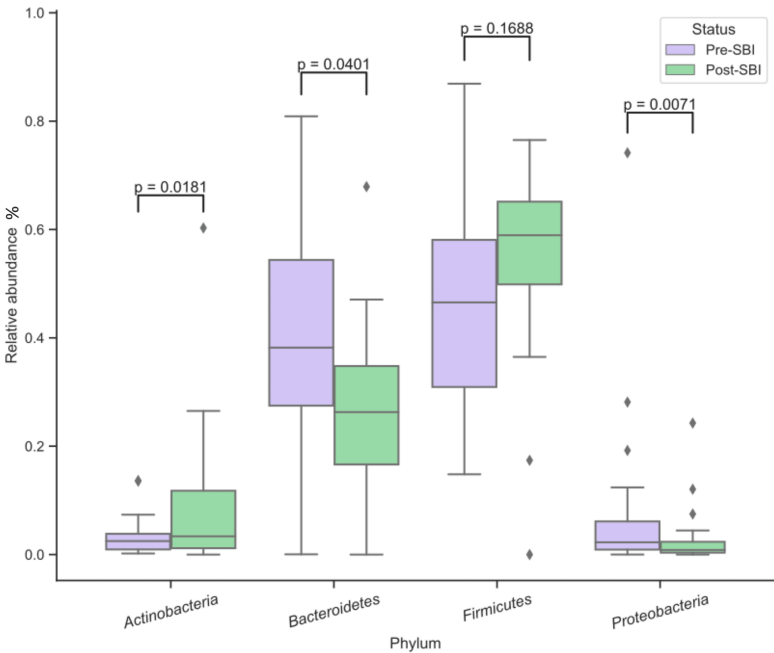
FIGURE 1: Relative abundances (%) of bacteria before and after SBI treatment at the phylum level.
