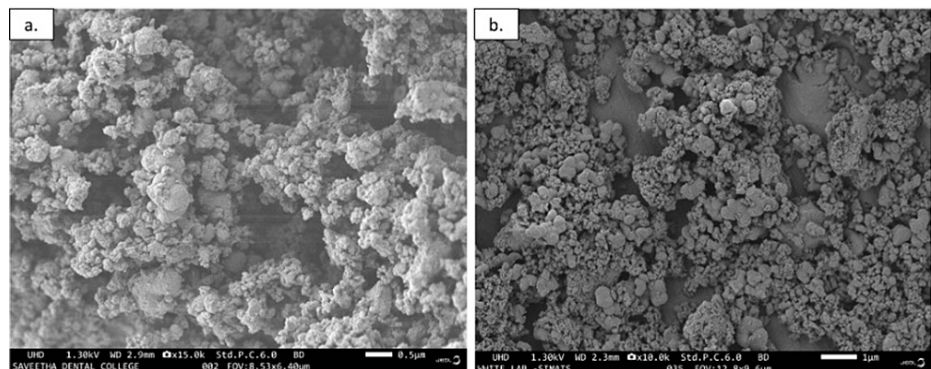
FIGURE 4: SEM micrograph of (a) M-TiO 2 NPs and (b) MCTN.
