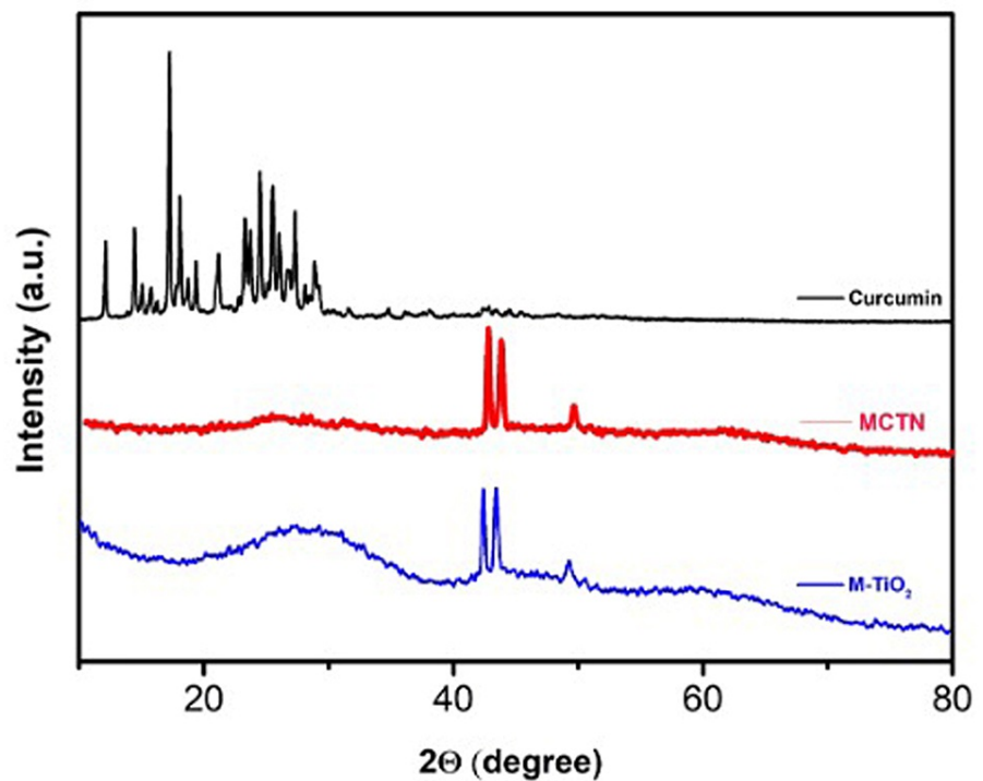
FIGURE 3: XRD pattern of Cur, M-TiO 2 NPs, and MCTN.
