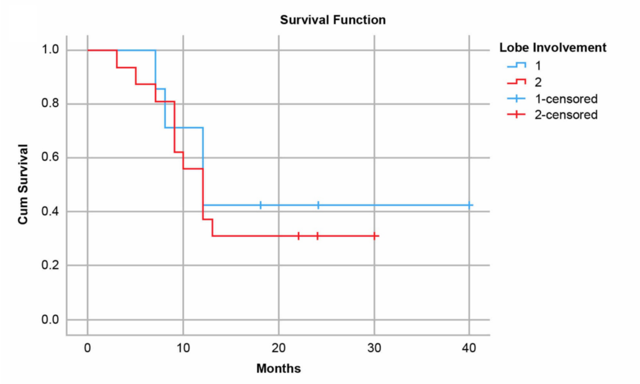
FIGURE 5: Kaplan-Meier curves for patients after undergoing transarterial radioembolization with resin microspheres for hepatocellular carcinoma or liver metastases showing survival by lobe involvement
