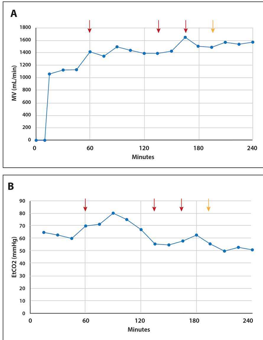
FIGURE 1: MV and EtCO2 in response to ascending dose of continuous infusion ENA-001
