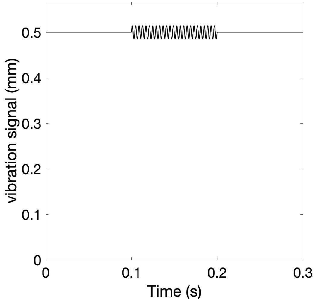
FIGURE 3: Vibratory burst at 250 Hz.
