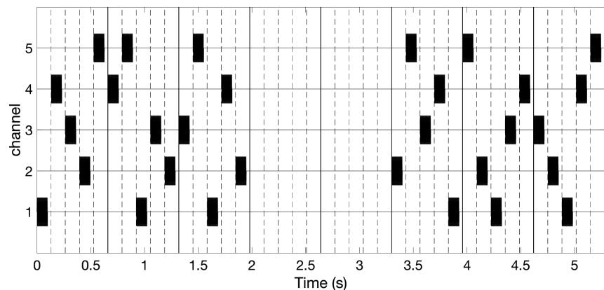
FIGURE 2: Burst-like vibrotactile coordinated reset stimulation with high-frequency of 250 Hz vibratory bursts (black rectangles) and vibrotactile coordinated reset stimulation period of 660 ms, delivered via five channels.
