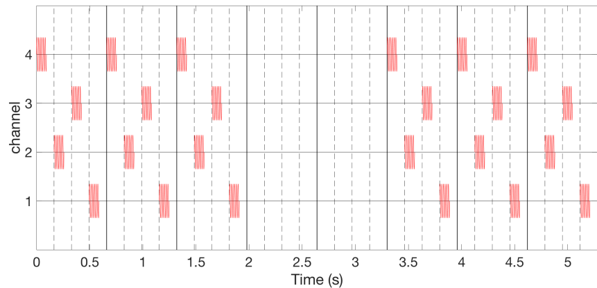
FIGURE 7: Burst-like vibrotactile coordinated reset stimulation with low-frequency of 64 Hz vibratory bursts and fixed vibrotactile coordinated reset stimulation sequences, delivered via four channels.
