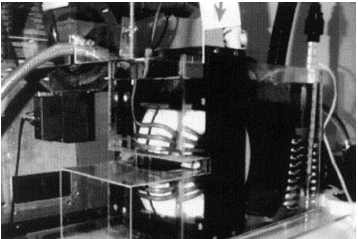
Figure 5: Early Prototype of AMF Administration Device
