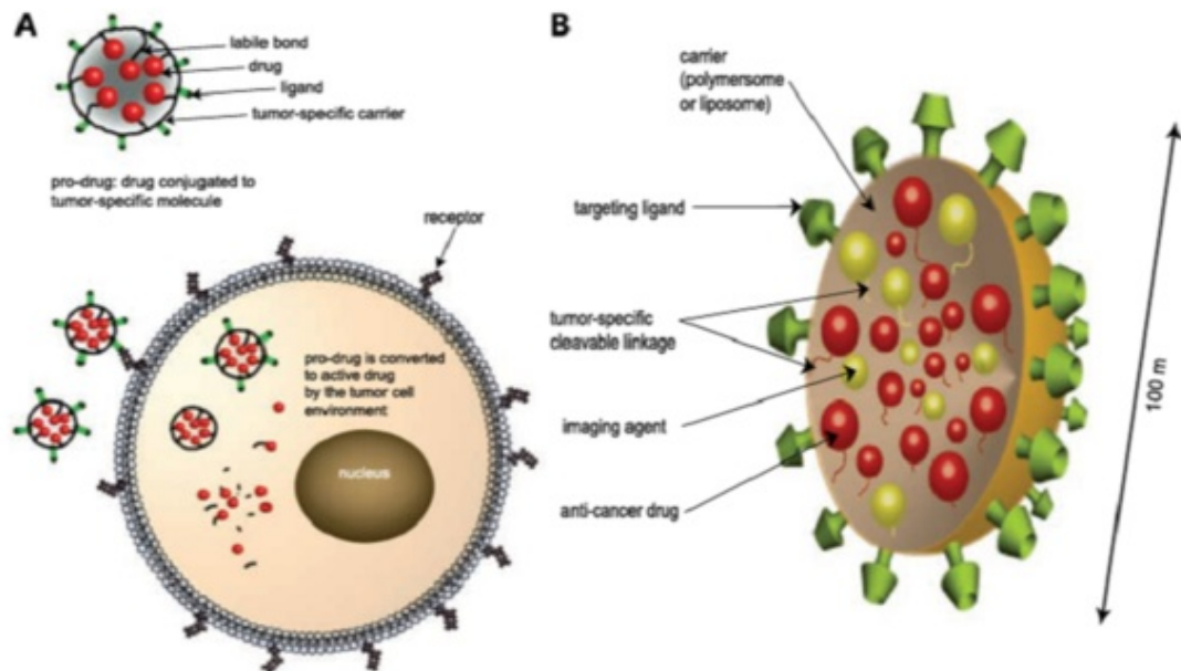
Figure 2: Nanoparticle Applications
